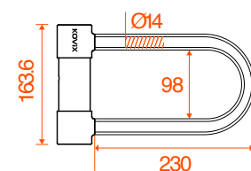
DIMENSIONS *ALL Dimensions in mm
