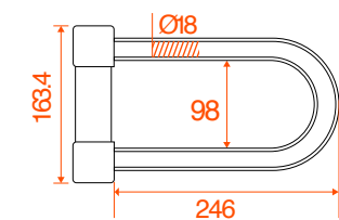
DIMENSIONS *ALL Dimensions in mm
